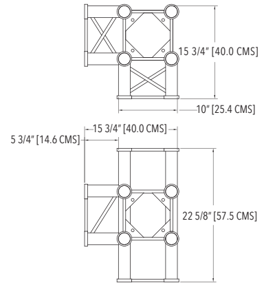
▶ TRL 010 TRUSS TEE W/D
